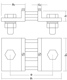
SHUNT 200-1000
