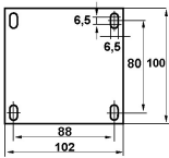
FIXING SUPPORT
