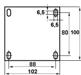
FIXING SUPPORT
